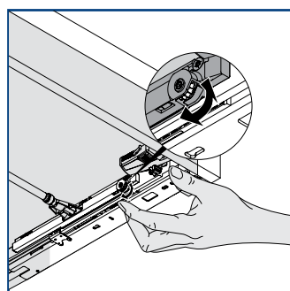
Depth adjustment +2/-1 mm for MOVENTO with TIP-ON
