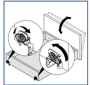
Tilt adjustment on back of runners
