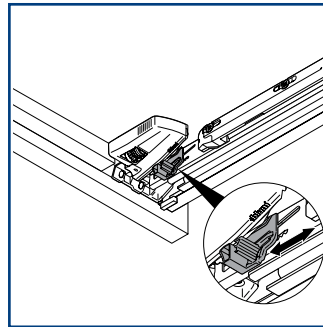
Height adjustment on both sides via locking device +3 mm
