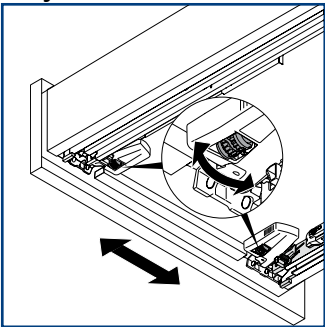
Side adjustment on both sides via locking device +/- 1.5 mm
