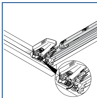
Depth adjustment +/- 2 mm for MOVENTO with BLUMOTION
