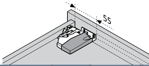
Drawer Assembly - Front
